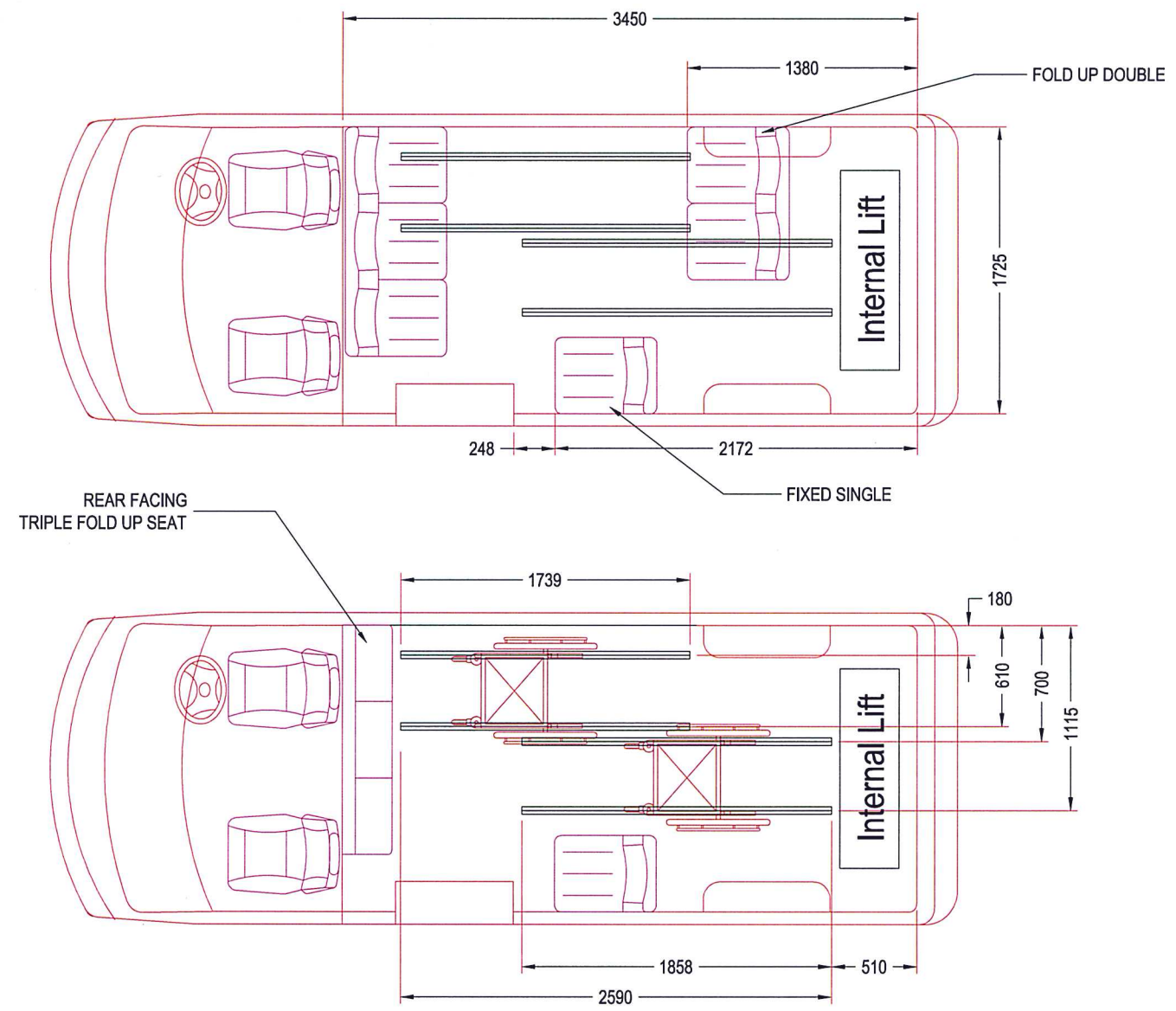
TITLE: TOYOTA COMMUTER SLWB - 7 SEATS PLUS DRIVER - 3 SEATS WITH 2 WHEELCHAIRS (REAR INTERNAL LIFT)
